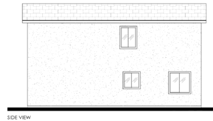
EXTERIOR ELEVATIONS - ADDITIONAL DWELLING UNIT
